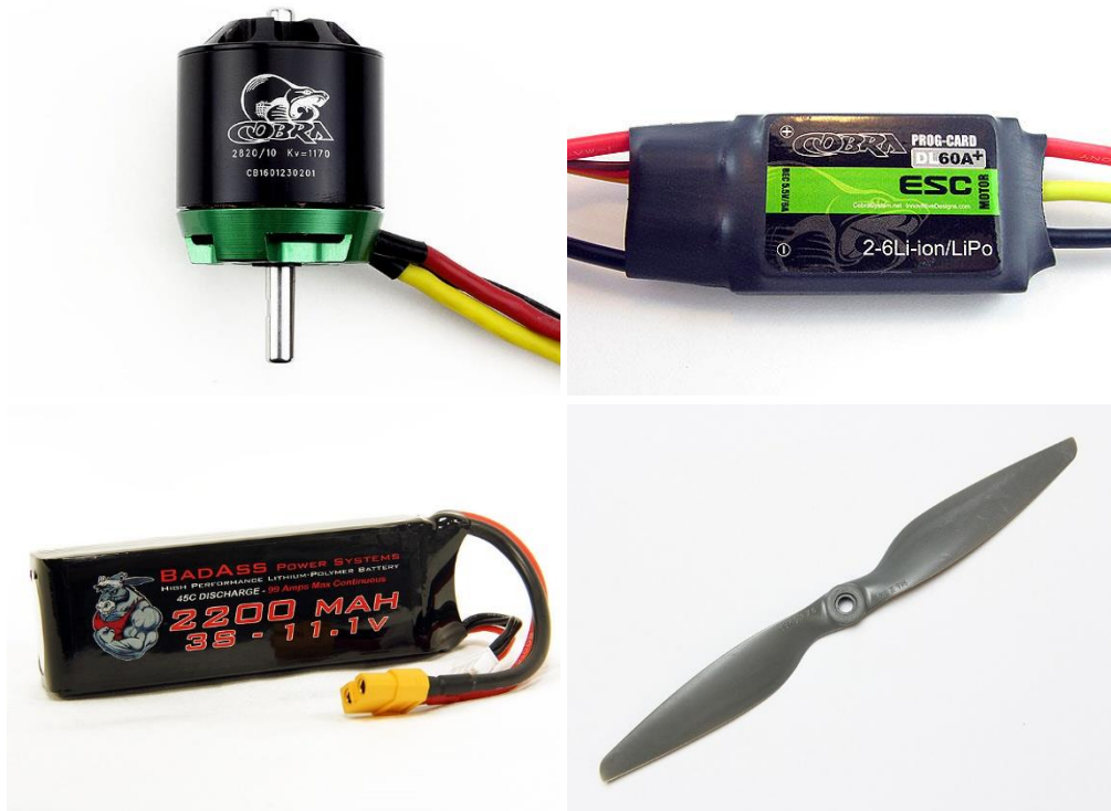
C-2820/10 1170Kv Motor, C-60A-ESC, APC 10X6 or 11x5.5 Prop on 3S 2200mah LiPo Battery
